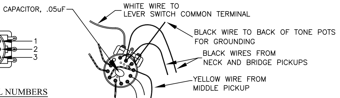
S-1 SWITCH WIRING DETAIL
