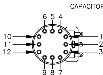
S-1 SWITCH TERMINAL NUMBERS
