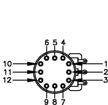
S-1 SWITCH TERMINAL NUMBERS
