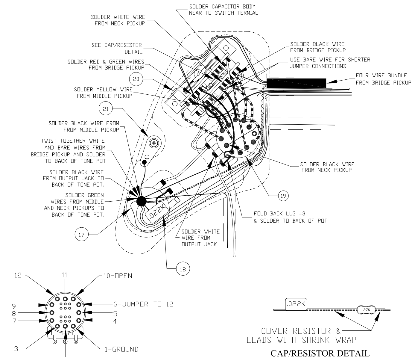
S-1 SW/POT TEREMINALS DETAIL
