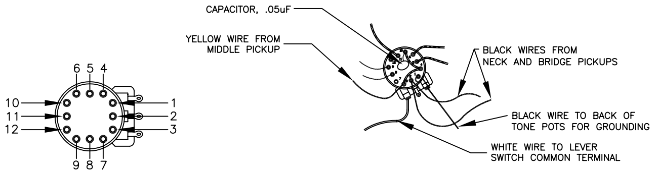
S-1 SWITCH TERMINAL NUMBERS
