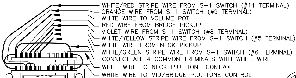
LEVER SWITCH WIRING DETAIL
