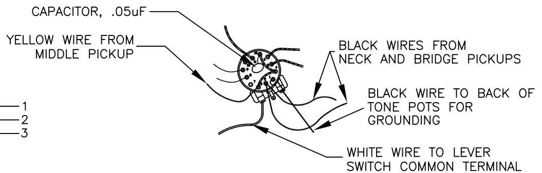
S-1 SWITCH TERMINAL NUMBERS
