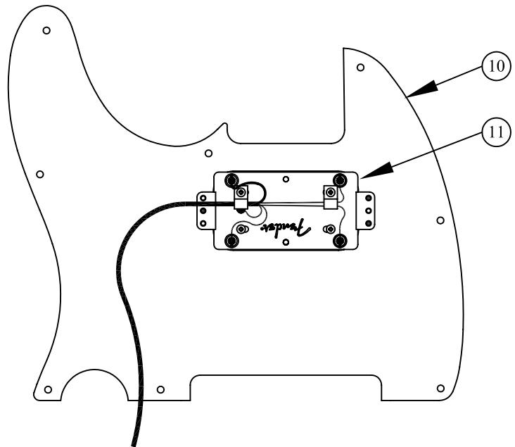
PICKGUARD ASSEMBLY
