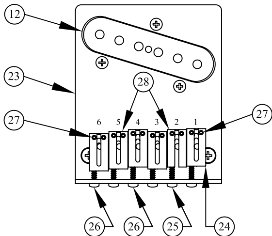
BRIDGE ASSEMBLY
