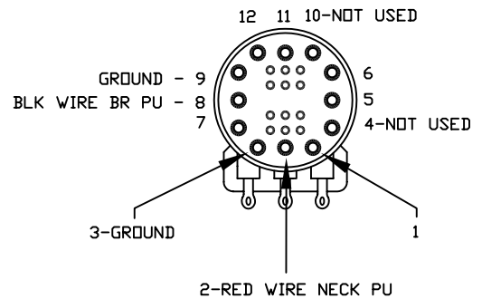
S-1 SWITCH WIRING DETAIL
