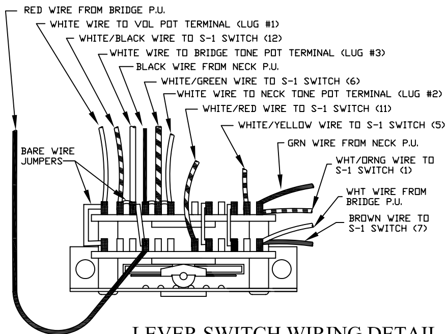
LEVER SWITCH WIRING DETAIL
