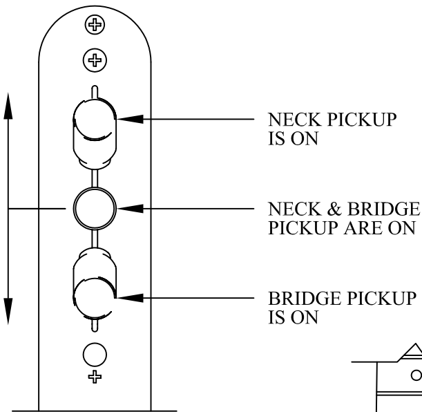
DETAIL 3 WAY SWITCH
