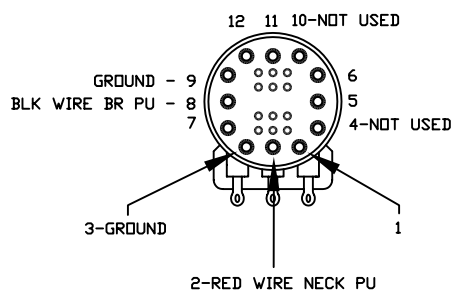
S-1 SWITCH WIRING DETAIL
