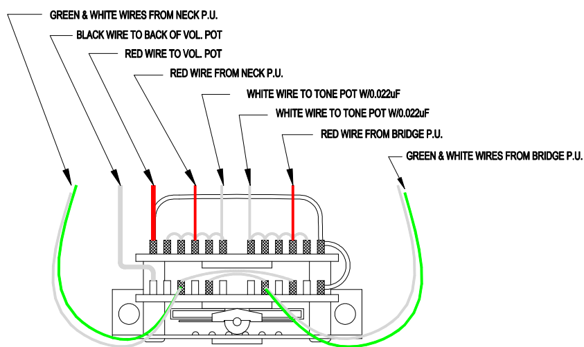
SWITCH WIRING DETAIL
